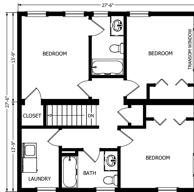
2nd Floor
