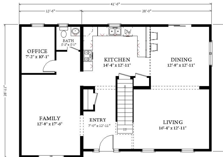
1st Floor
