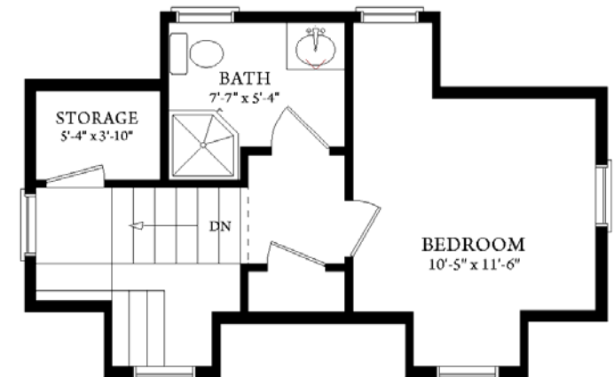
Proposed 2nd Floor (To be Finished Onsite)
